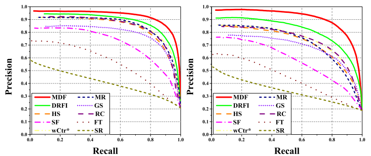
Figure 2: Precision-recall curves of 10 different methods, including ours (MDF), on two datasets: (Left) the MSRA-B dataset, and (Right) our new dataset (HKU-IS). Our method consistently outperforms other methods, including spectral residual (SR), frequency-tuned saliency (FT), saliency filters (SF), geodesic saliency (GS), hierarchical saliency, regional based contrast (RC [1]), manifold ranking (MR [4]), optimized weighted contrast (wCtr* [5]) and discriminative regional feature integration (DRFI [2]).
